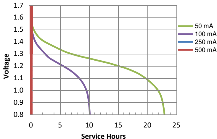
Constant Current
