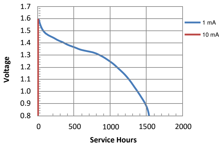
Constant Current
