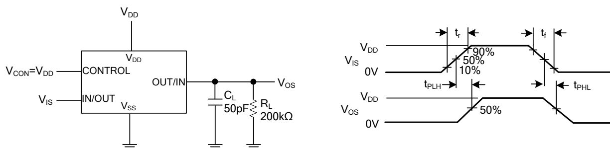
Fig. 1 t_{PLH} , t_{PLH} Propagation Delay Time Signal Input to Signal Output
