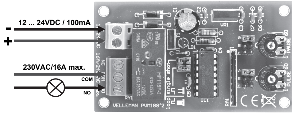
CONNECTION EXAMPLE: AC POWER (230VAC)
