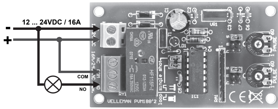
CONNECTION EXAMPLE: LOW VOLTAGE (12 ... 24VDC)
