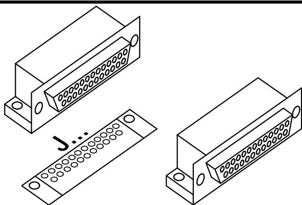
J5: 25P SUB-D, FEMALE ! (Connection: TO PC-SCOPE)
