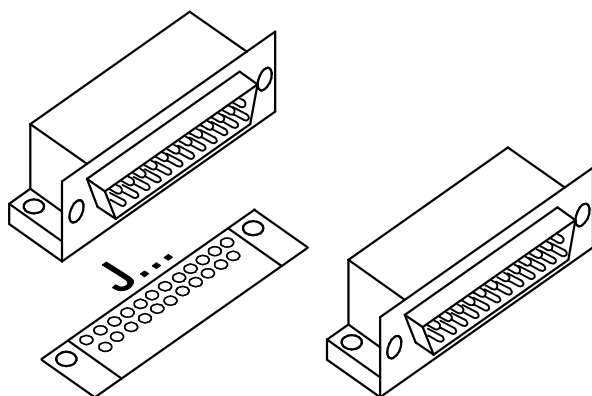
J7: 25P SUB-D, MALE ! (Connection: FROM PRINTER PORT)
