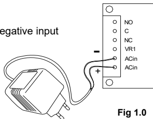
ADAPTER (16-18VDC/100mA)
